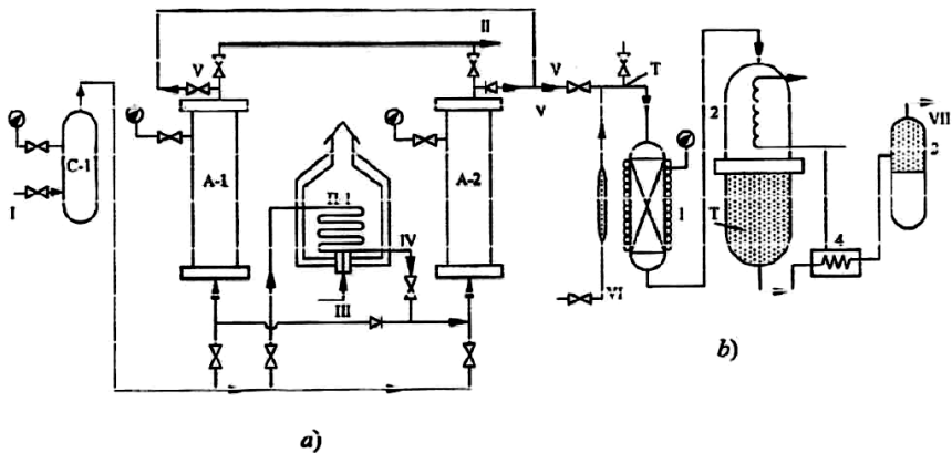
Fig. 1. Technological scheme of hydrogen sulfide adsorption from low sulfurous natural gases and its conversion into elemental sulfur: A-1, A-2 – adsorbers; C-1 – separator; P-1 – furnace; I – converter with catalyst; 2 – coagulator; 3 – sulfur trap; 4 – cooler. Flows: I – raw gas; II – pure gas; III – fuel gas; IV – regenerating gas; V – desorption products; a) adsorption unit; b) reactor section
